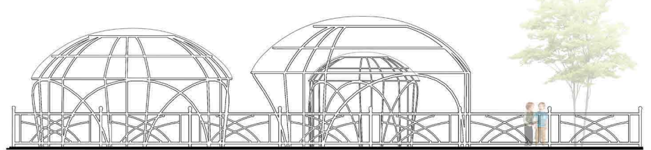
Cut B - B1 Scale 1:30
