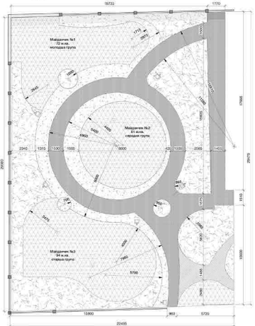
Plan Scale 1:100
